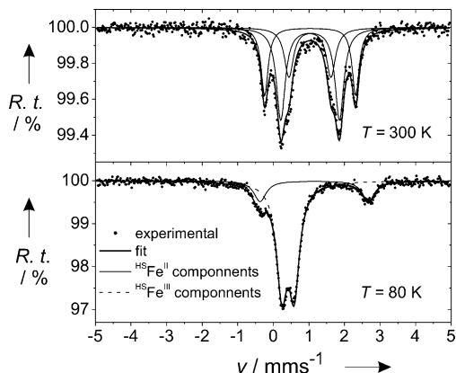
Figure 4. The Mössbauer spectra of \mathbf{1}^{\text{HT}} (top) and \mathbf{1}^{\text{T}} (bottom).
